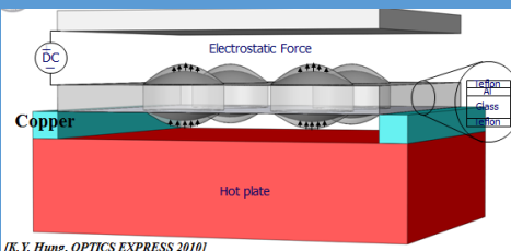
The design concept of the Double Aspheric Lens
