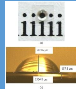
Micro aspheric lens
