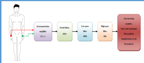
Portable ECG
