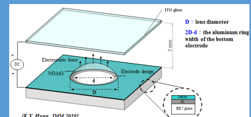
The design concept of the Hybrid Aspheric Lens
