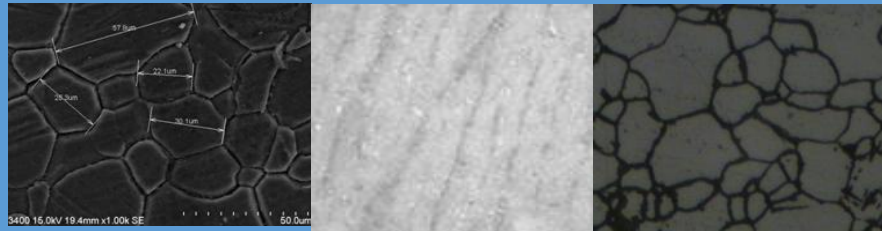
Phase transformations in Mg-Sn alloy
