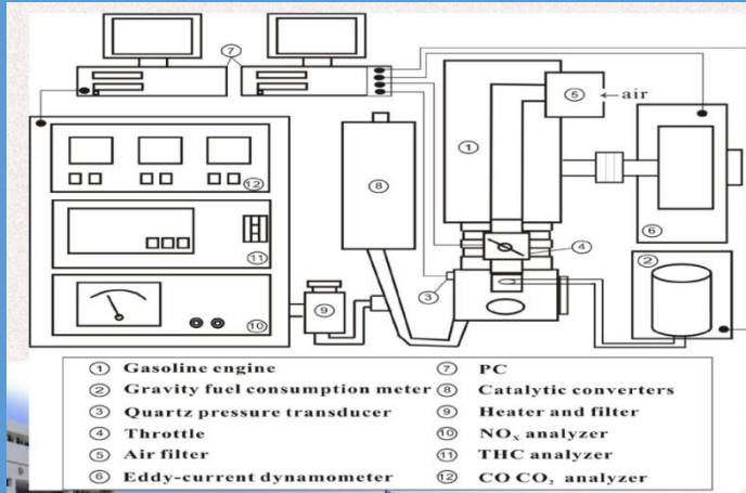
Powertrain-Laboratory structure
