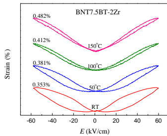
Hysteresis loops of strain vs. E-field in lead-free piezoelectric ceramics
