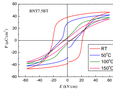
Temperature dependence of polarization hysteresis loops in ferroelectric ceramics
