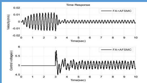
control of pneumatic vibration-isolation system
