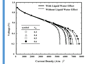
PEMFC and its performance
