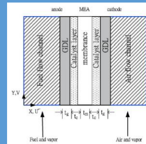
PEMFC and its performance
