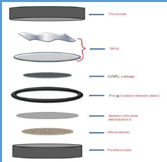
Assembly of lithium coin cell
