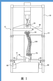
Spine tester with pure torque
