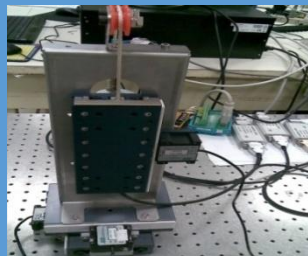
3D piezo-actuated system
