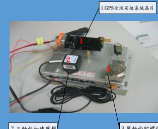
GPS/INS integration system
