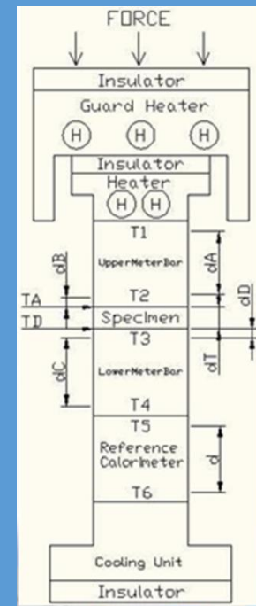
Thermal Interface Material Measurement Apparatus
