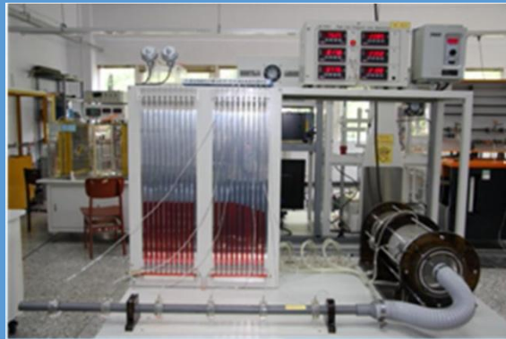
Pipe friction factor and valve characteristic measurement Apparatus
