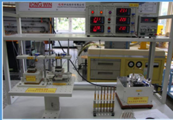
Heat pipe characteristic measurement Apparatus
